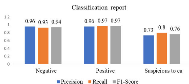
Figure 6: Report on classification results for the test set before preprocessing
